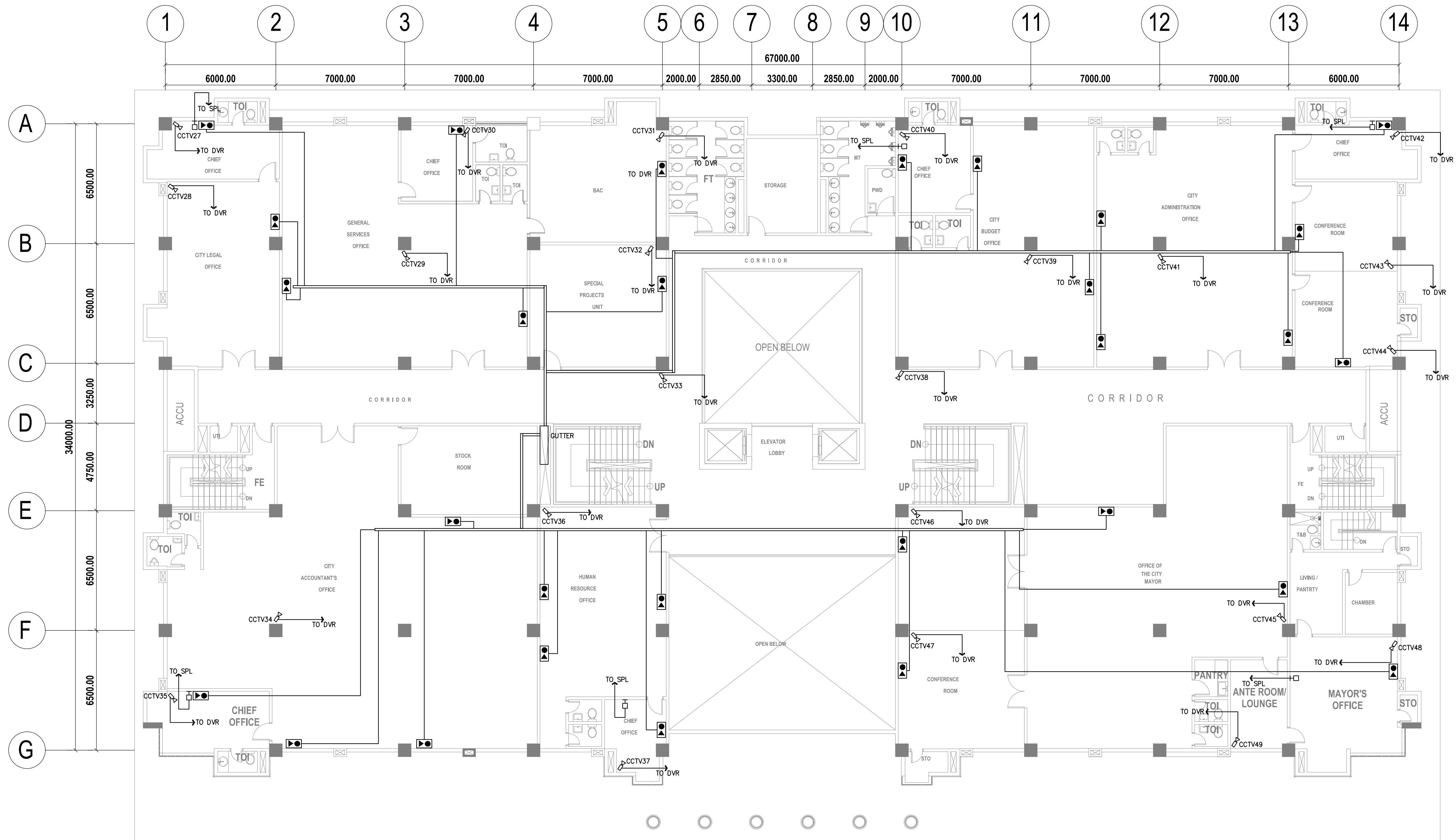
1 SECOND FLOOR AUXILIARY LAYOUT E-13 SCALE 1:125
